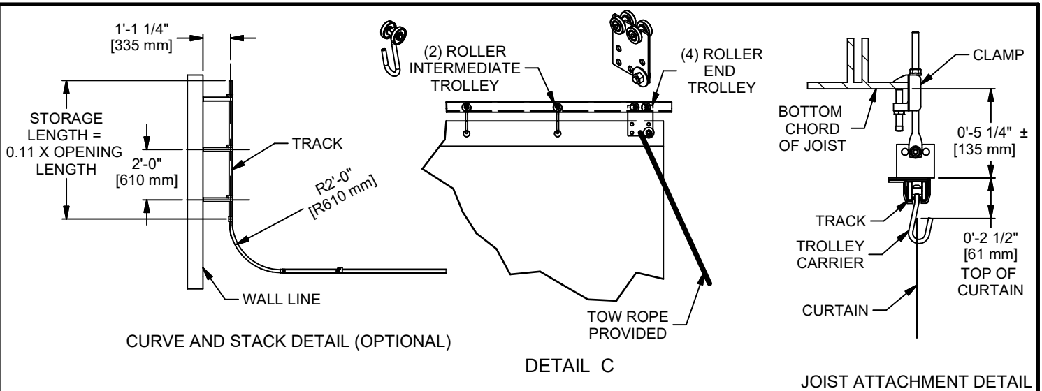
JOIST ATTACHMENT DETAIL
