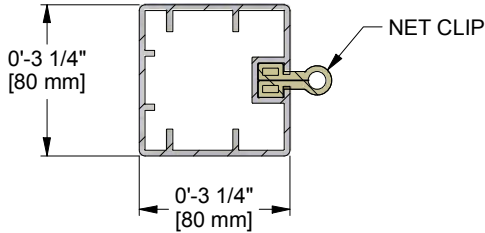
SECTION A-A ALUMINUM EXTRUDED FRAME MEMBER
